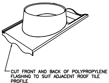
3D FLASHING VIEW - DETAIL D SCALE N.T.S.
