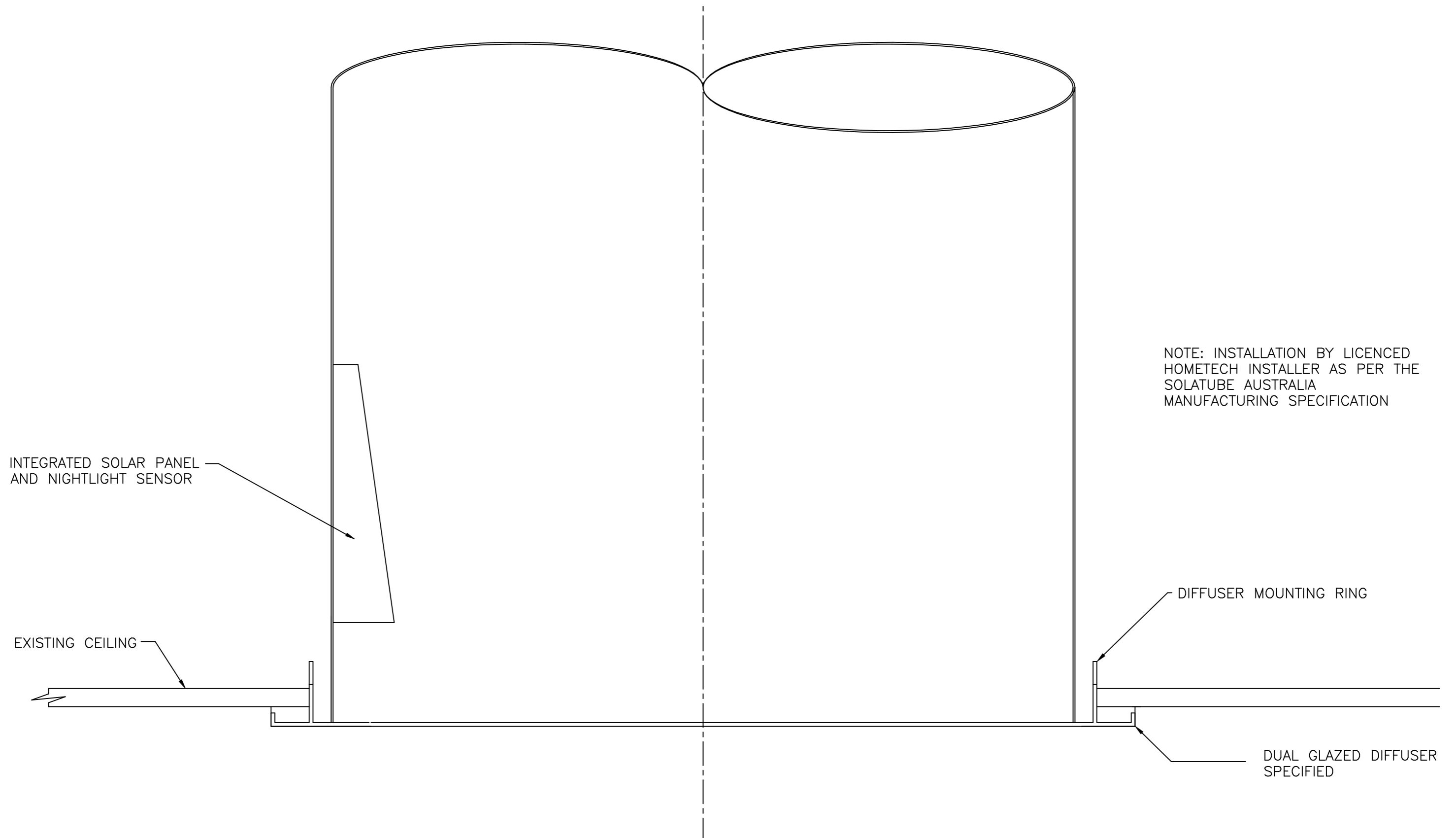
SECTION THROUGH ELECTRIC LIGHT DAMPER SCALE 1:5
