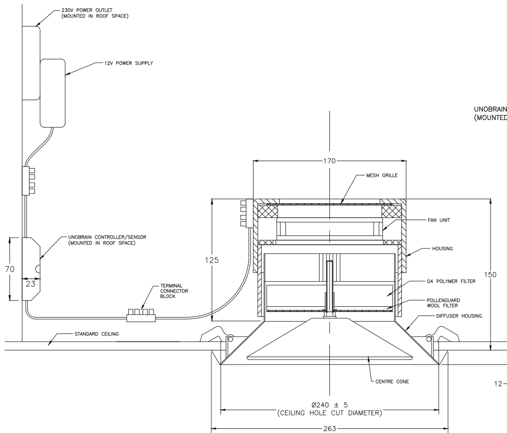
CROSS SECTION THROUGH CEILING
